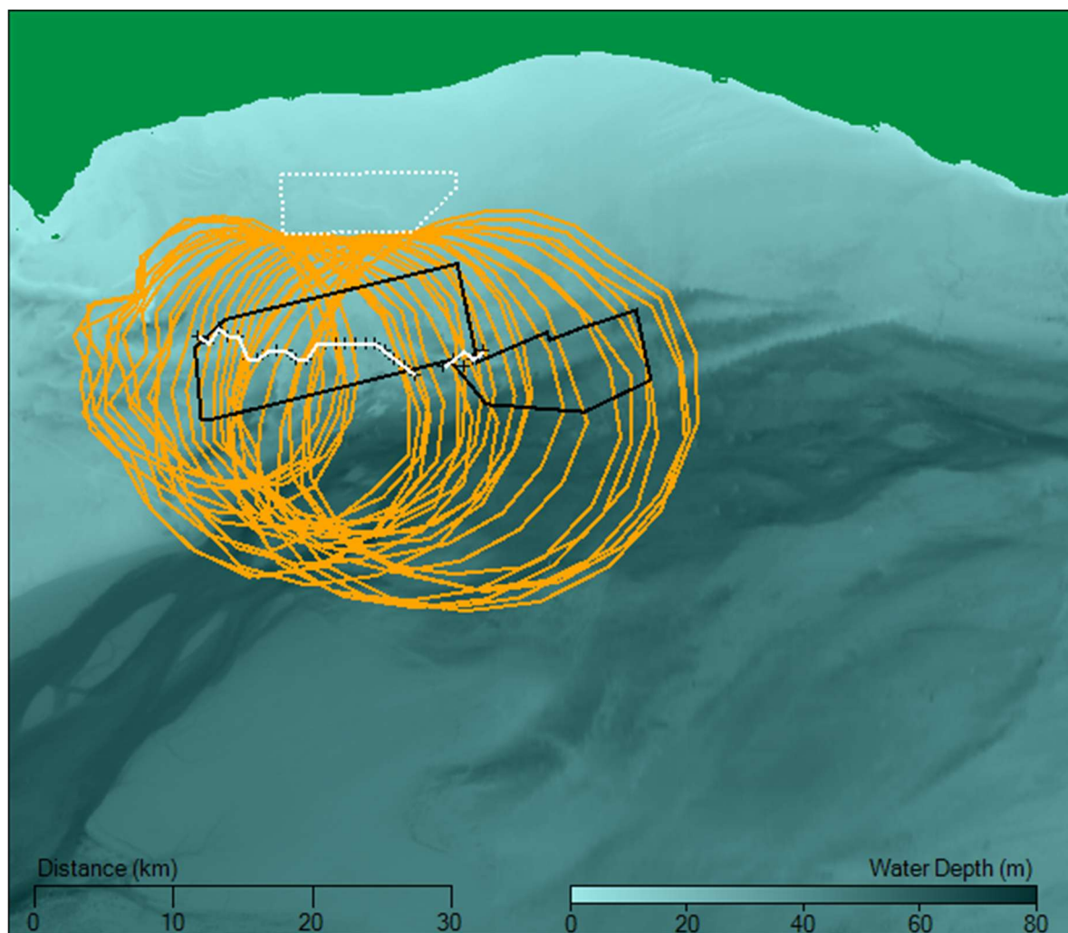
Figure 5.5 Mitigated multileg foundation piling impact contours (141dB re 1 \mu\text{Pa}^2\text{s} (SELss)) used to define piling exclusion zones (DBBC) (15dB reduction)
