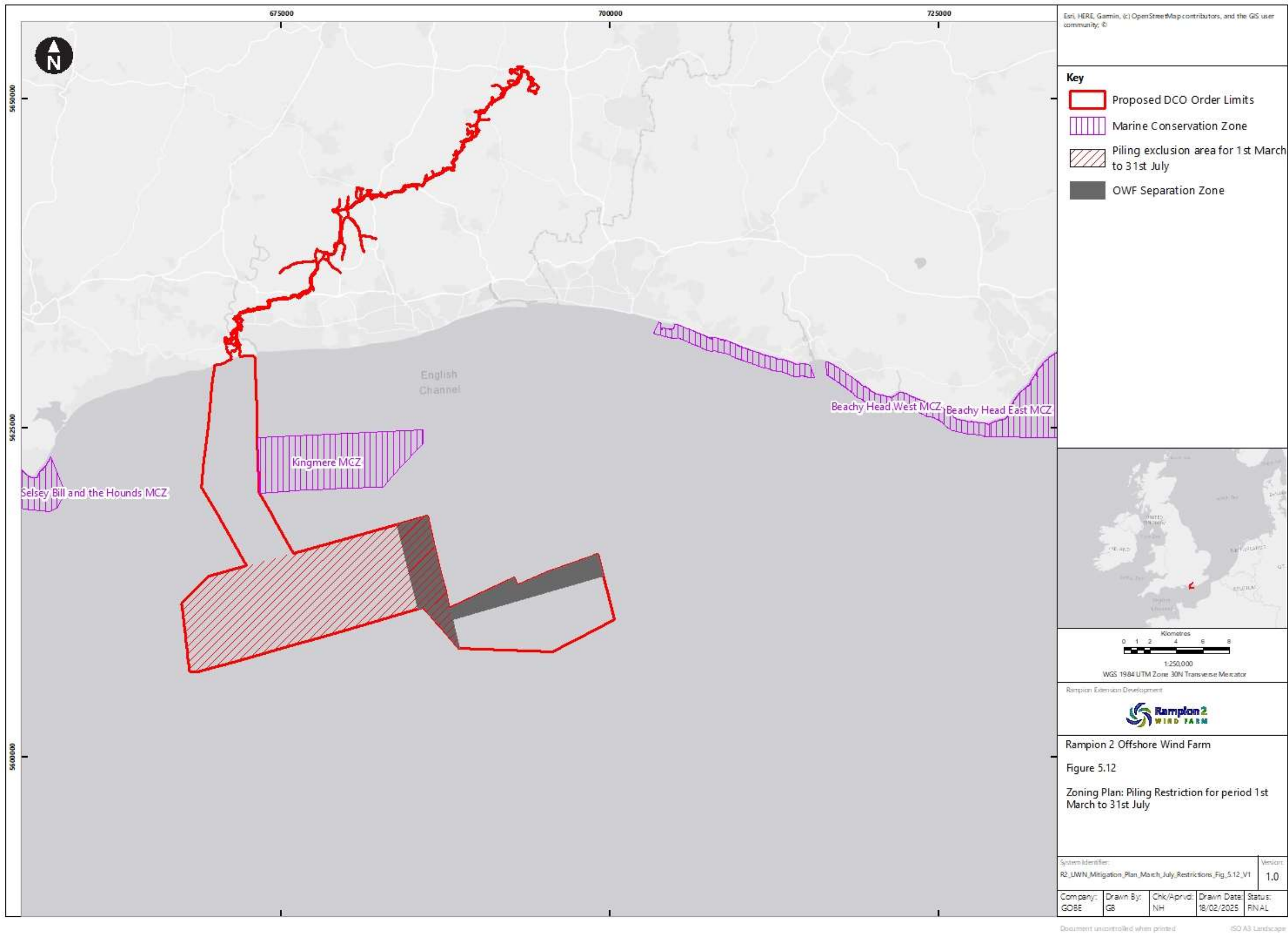
Figure 5.12 Zoning Plan: Piling Restriction for period 1 st March to 31 st July
